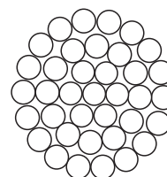
37 Al.Alloy
