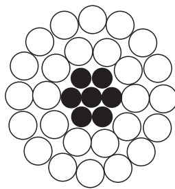
26 Al. 7 Steel
