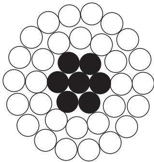
30 Al. 7 Steel
